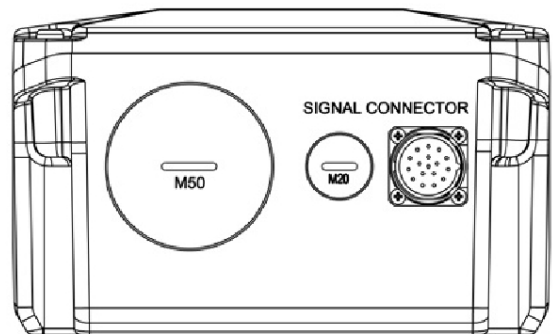
接线盒 175×175 CONNECTION BOX 175×175
